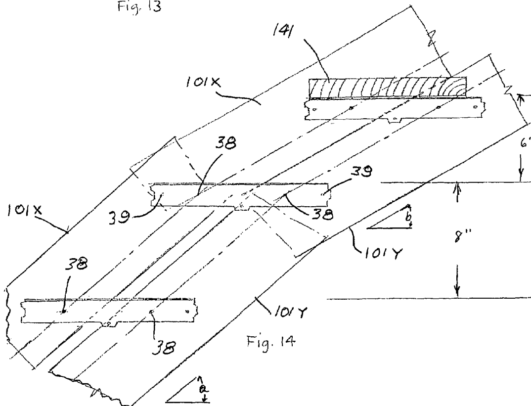
LOADING BRACKETS ON STRINGER EDGE TO MARK BRACKET SPACING CENTERS "X"
